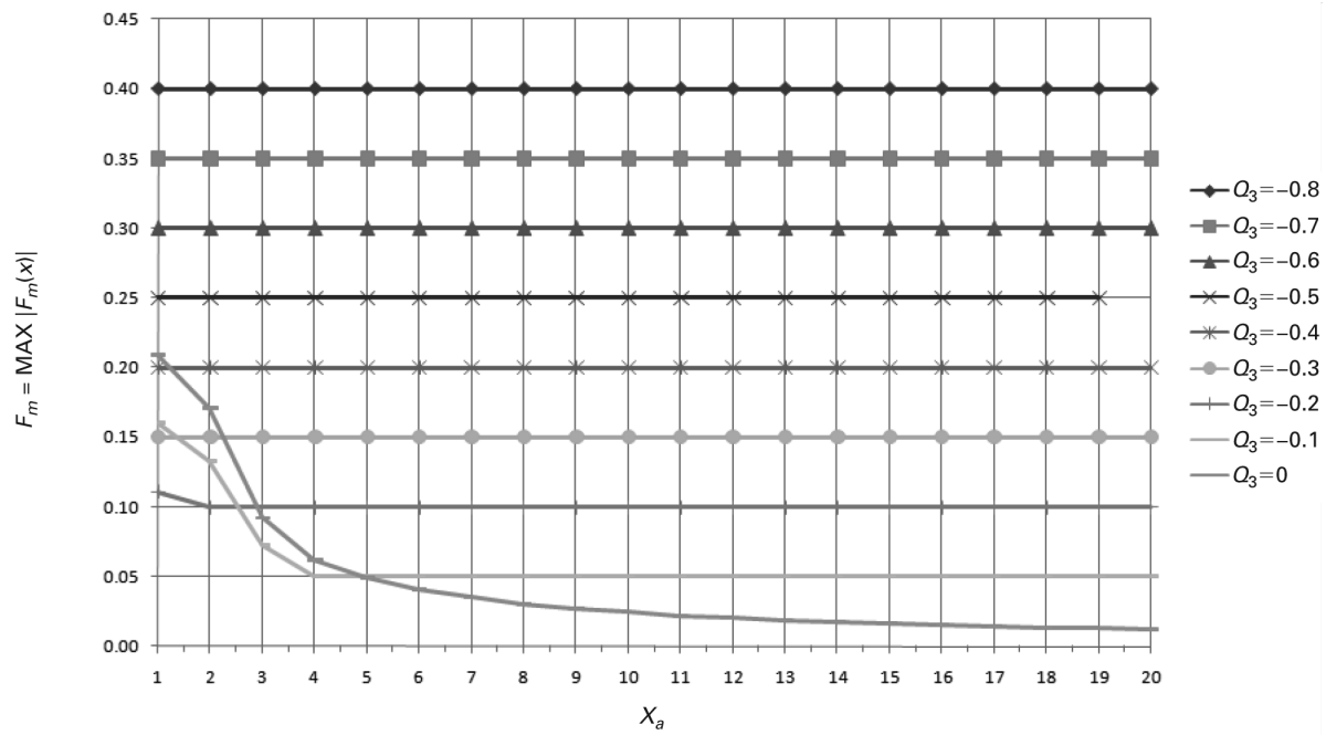
Figure LL-1-2 F_m Versus X_a and Q_3 ( -0.8 \leq Q_3 \leq 0 )
