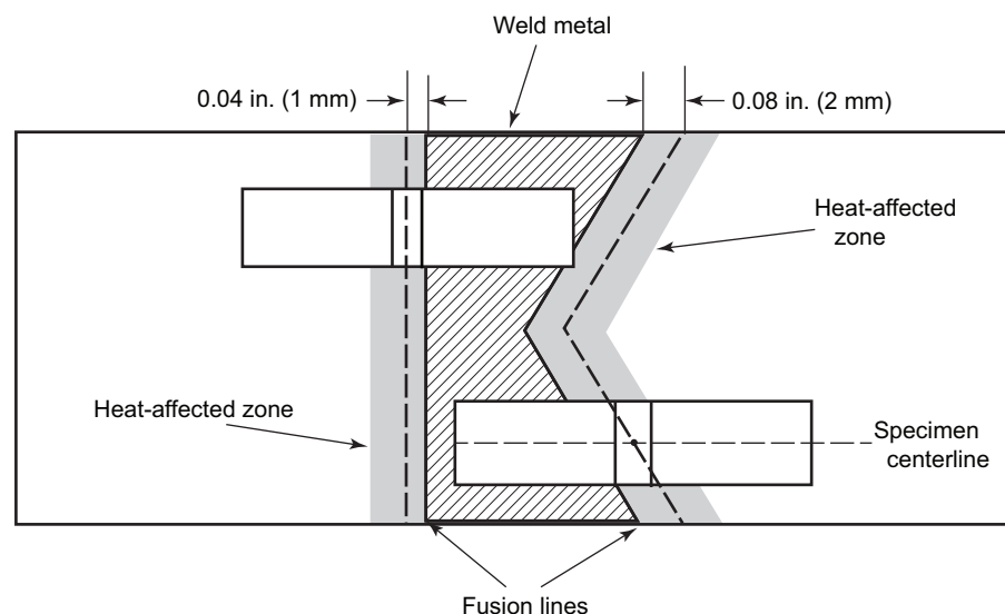
Figure UG-84.6 Location of HAZ Specimen Removal
