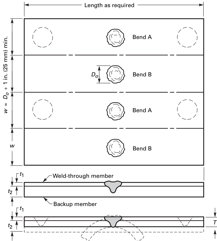
Figure 17-12 Gas Metal Arc-Spot-Weld Block for Bend Tests
