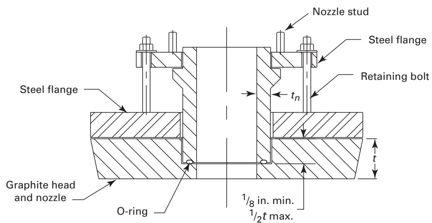
(e) O-Ring
