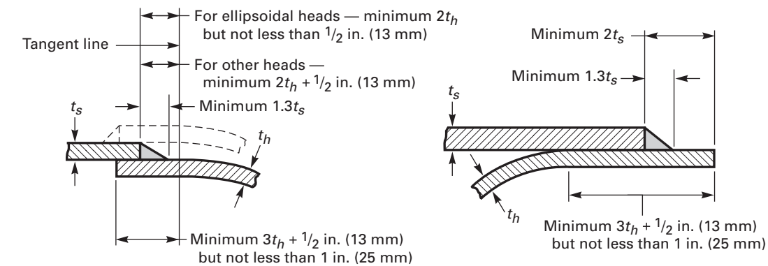
(a) Single Fillet Lap Weld
