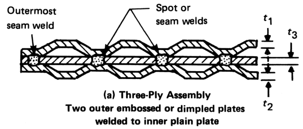
Figure 17-6 Three-Ply Assemblies
