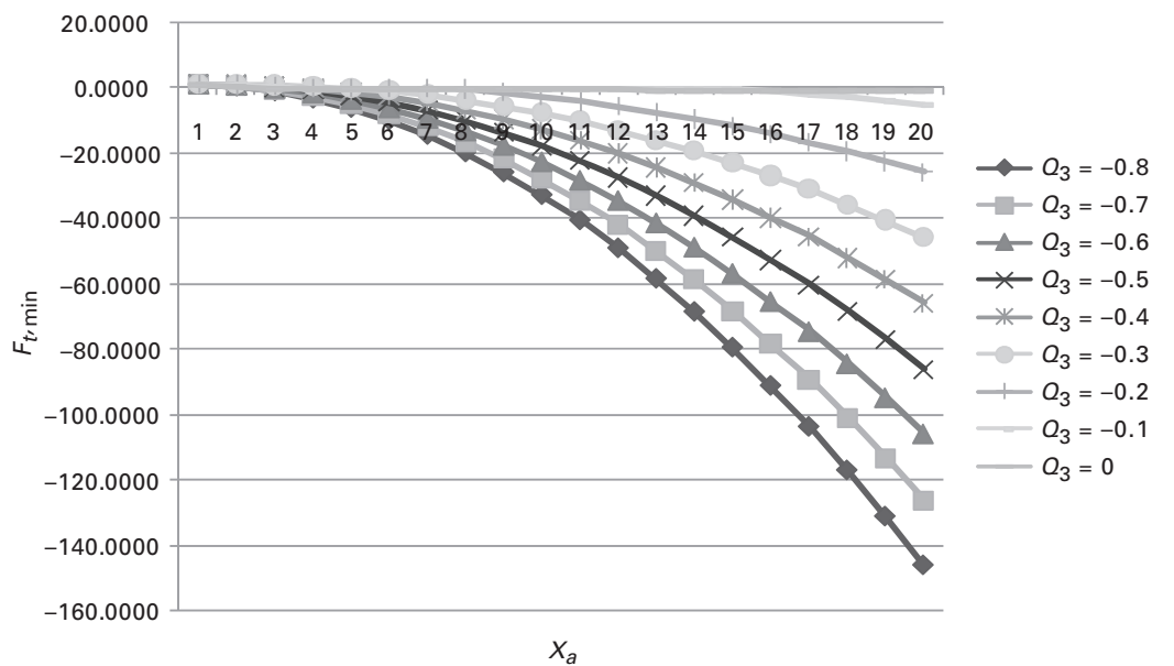
Figure LL-1-3 Graphical Representation of F_{t,min}
