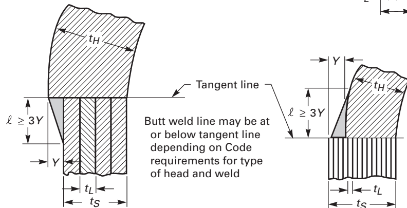
(e) For Layers 5/8 in. (16 mm) or Less in Thickness [See Note (2)]
