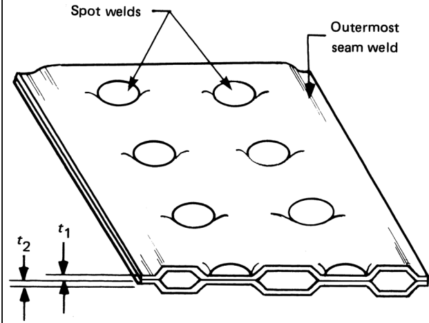
Figure 17-2 Two Dimpled Plates
