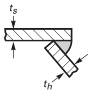
(f-1) Not Permissible
